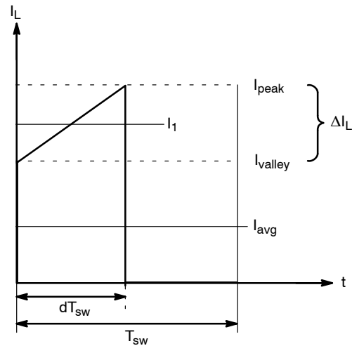
Figure 46. Primary Inductance Current Evolution in CCM
